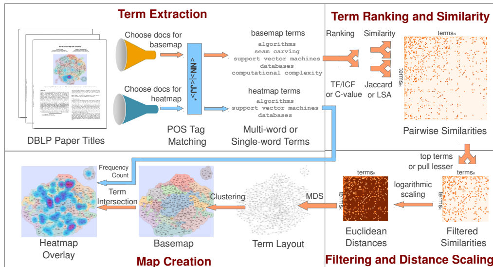
Figure 2: The main steps of the MoCS system are querying documents from DBLP, extracting terms from these titles, ranking terms by importance, calculating term similarity, further filtering terms based on similarity, and finally performing multidimensional scaling and clustering to produce a basemap, over which a heatmap can be overlaid.
